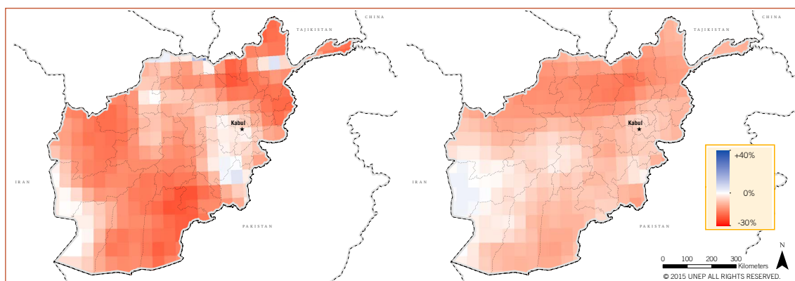
Figure 17: Projected Changes of Annual Precipitation in % for Afghanistan as Mean of Seven Regional Climate Models Between a Scenario Period (2021-2050) and a Base Period (1976-2005) Under Limited GHG Emissions (left, RCP 4.5) and Uncontrolled GHG Emission (right, RCP 8.5).
