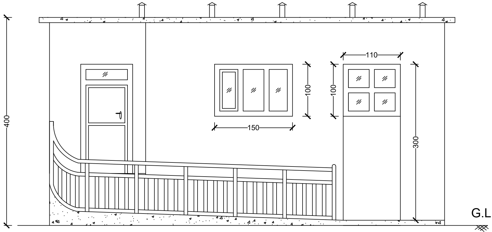
Front Elevation
