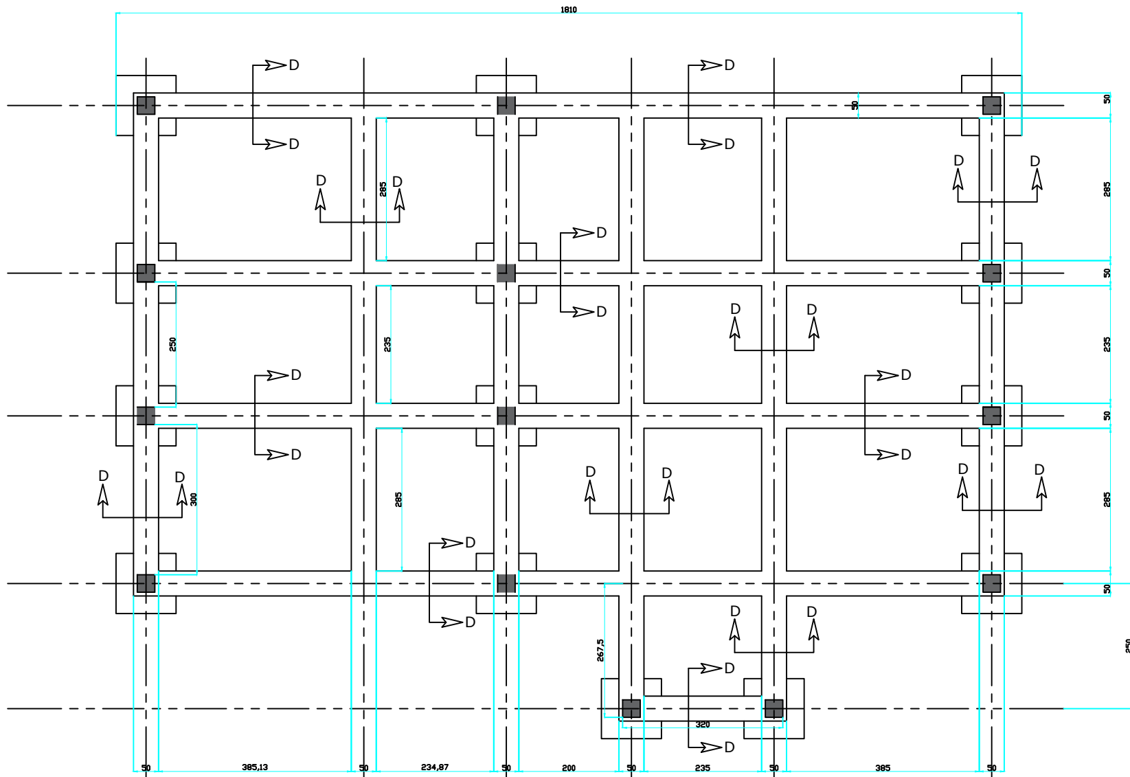
Stone Masonry Footing Plan
