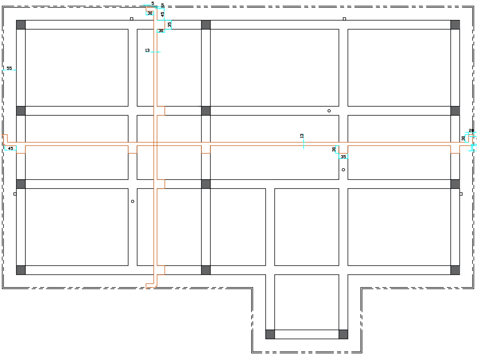
Forming plan of Roof Slab
