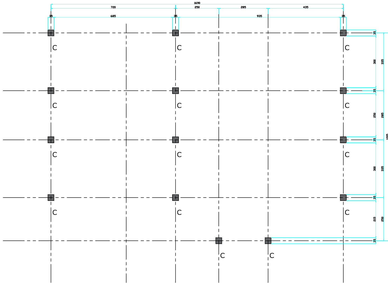
RCC Column Plan
