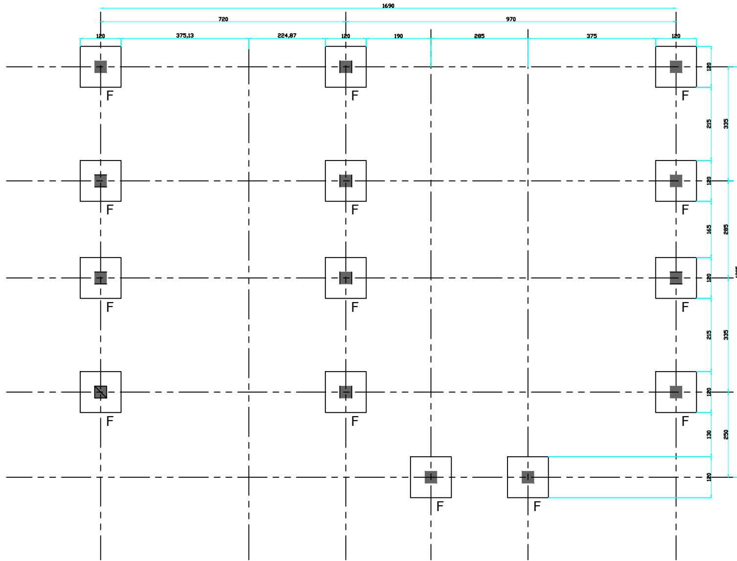
RCC Footing Plan
